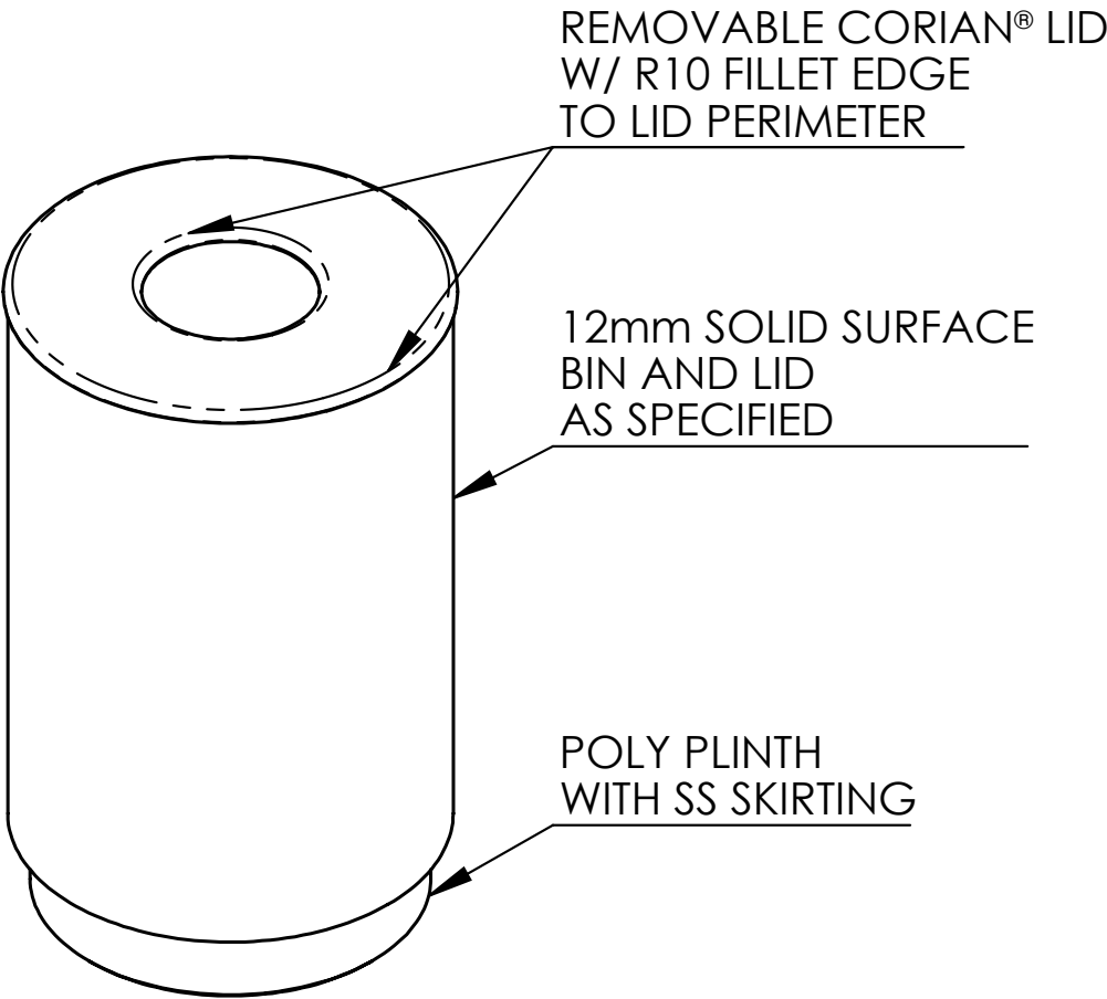
ISOMETRIC VIEW
