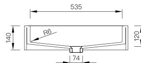
CROSS-SECTION
