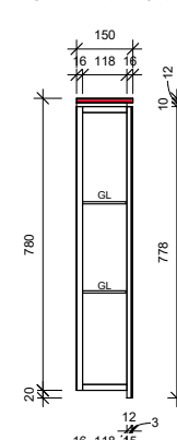
ALL PANEL SIDE ELEVATION
