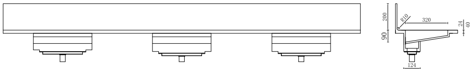
CROSS-SECTION
