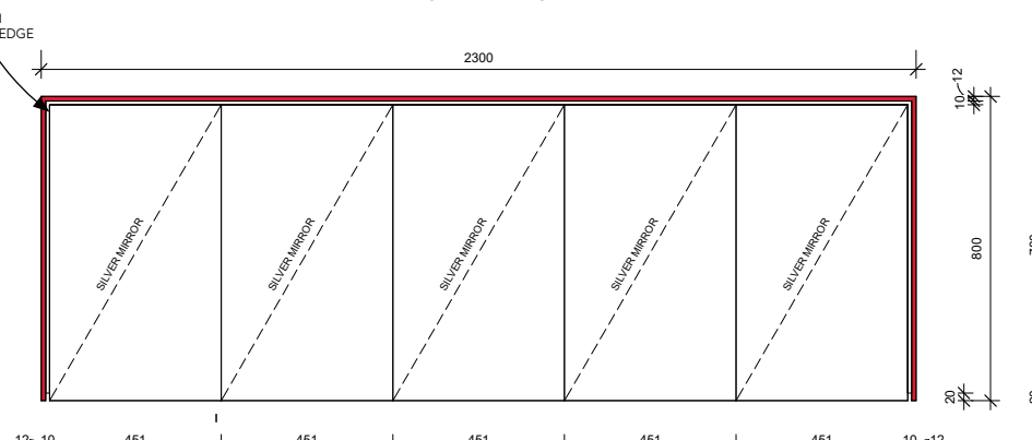
5 PANEL FRONT ELEVATION
