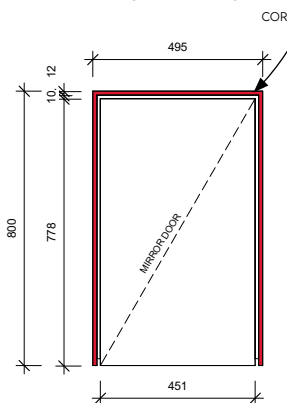
1 PANEL FRONT ELEVATION
