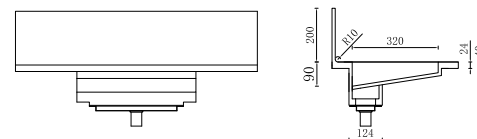
CROSS-SECTION
