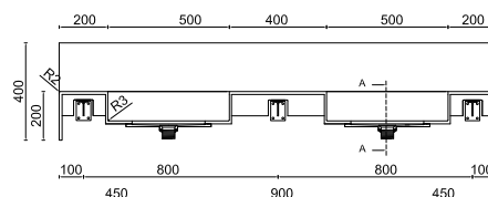
CROSS-SECTION
